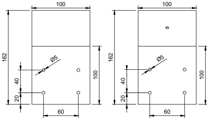
Expansion Bracket
