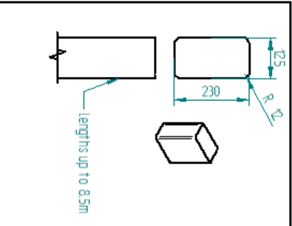
WHF571 Wharf fender 125 x 230mm Grey
