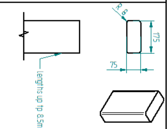
WHF075 Wharf fender 75 x 175mm Grey
